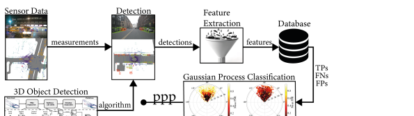
Figure 5: Data flow for the entire benchmarking process [1].
