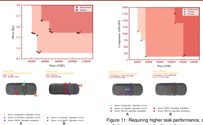
Figure 10: More expected obstacle configurations in a task increase resource requirements [1].
